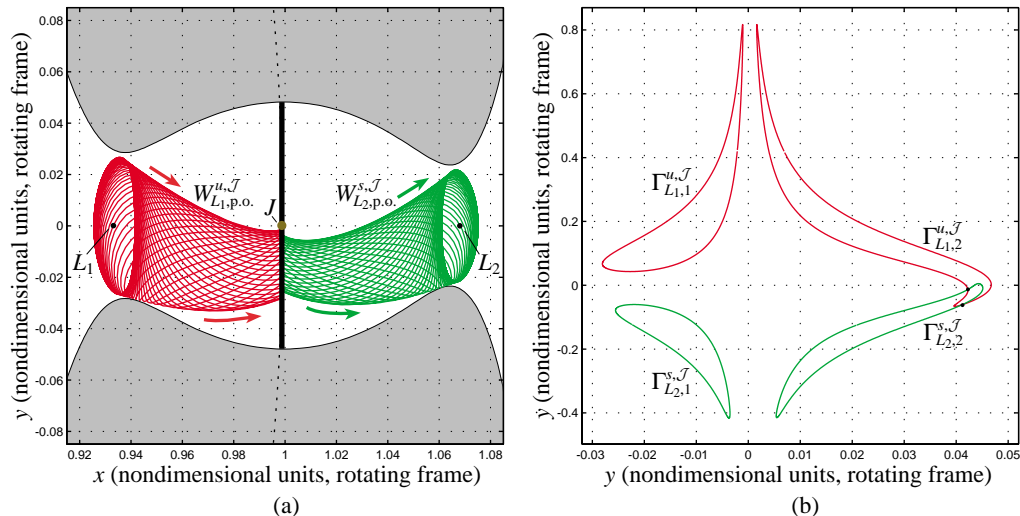
Figure 3.13: (a) The projection of invariant manifolds W_{L_1,p.o.}^{u,\mathcal{J}} and W_{L_2,p.o.}^{s,\mathcal{J}} in the region J of the position space. (b) The first two Poincaré cuts of the invariant manifolds with the plane x = 1 - \mu .
