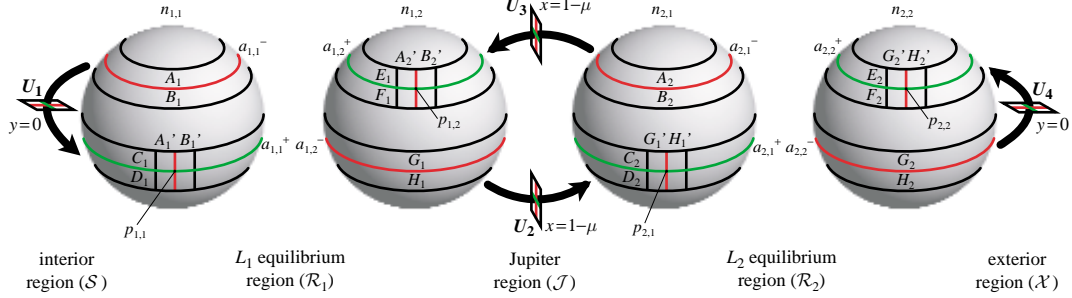
Figure 4.2: The strips near the asymptotic sets on the spheres n_{1,1}, n_{1,2}, n_{2,1}, n_{2,2} .
