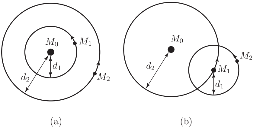
FIGURE 5.2.1. Models of motion for the four-body problem. (a) Concentric Circular Model. M_0 is a central body about which M_1 and M_2 move in circular orbits of radii d_1 and d_2 , respectively, where d_2 > d_1 . (b) Bicircular Model. M_1 and M_2 are in circular motion about their barycenter, with mutual separation d_1 . Considering all the mass in the M_1 - M_2 system to be concentrated at its barycenter, we suppose M_0 and the M_1 - M_2 barycenter are in a circular orbit of radius d_2 > d_1 about their common center of mass.
