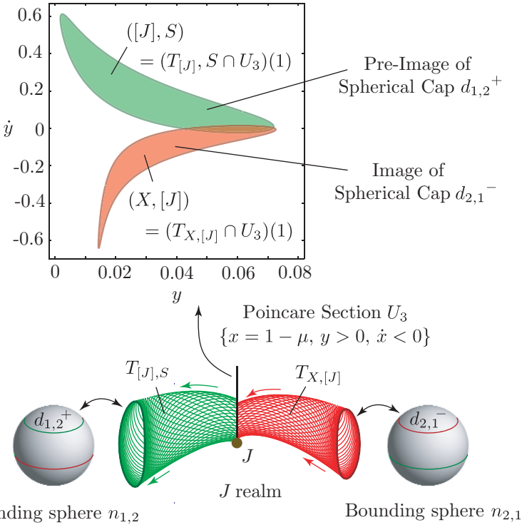
FIGURE 4.4.4. We seek transit orbits from the exterior to interior realm by looking at the intersections of images and pre-images of the “caps of transit orbits,” introduced for the equilibrium regions in Chapters 2 and 3. See the text for an explanation.
