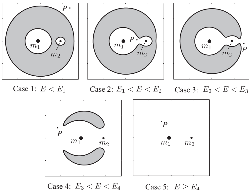
FIGURE 2.4.2. Realms of possible motion. Zero velocity curves for five values of the energy, one in each of the cases as described in the text, are shown on the x - y plane for \mu = 0.1 . These curves bound the zone, in white, accessible by the particle, P , for a given energy value, E = e . The part of the x - y plane which is shaded is inaccessible for a given energy, and known as the forbidden realm . The outermost accessible realm, known as the exterior realm , extends to infinity. In the case 5, the forbidden realm vanishes and motion over the entire x - y plane is possible.
