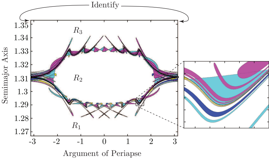
FIGURE 10.3.4. Transport across a resonance. The lobes formed by both the upper and lower boundaries of a resonance region R_2 are shown. Using the lobe dynamics framework, the transport of points between these regions can be computed systematically. An enlargement of the boxed region is shown at right.
