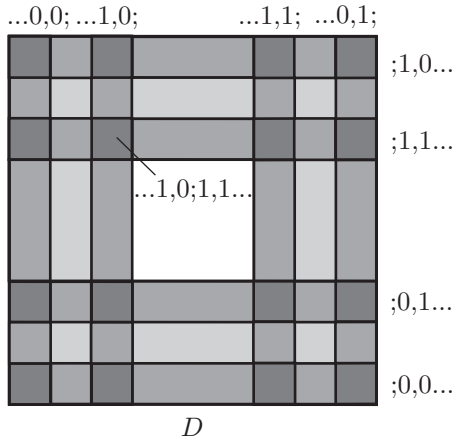
FIGURE 3.9.1. The invariant set \Lambda_h of the horseshoe map h .
