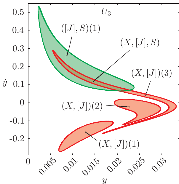
FIGURE 4.5.1. The first intersection of T_{[J],S} and the first three intersections of T_{X,[J]} with U_3 are shown. We use the notation (X, [J])(n) = (T_{X,[J]} \cap U_3)(n) for the n th intersection of T_{X,[J]} with U_3 . The intersection (X, [J], S) = (X, [J])(3) \cap ([J], S)(1) contains all solutions s(t) which come from the X realm, perform two full revolutions around Jupiter in the J realm, and then exit to the S realm.
