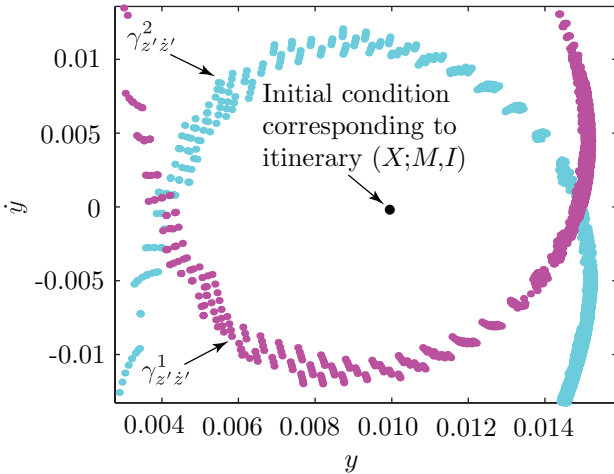
FIGURE 9.4.5. On the (y, \dot{y}) -plane are shown the points that approximate \gamma_{\dot{z}', \dot{z}'}^2 and \gamma_{\dot{z}', \dot{z}'}^1 , the boundaries of \text{int}(\gamma_{\dot{z}', \dot{z}'}^2) and \text{int}(\gamma_{\dot{z}', \dot{z}'}^1) , respectively, where (z', \dot{z}') = (0.0035, 0) . Note the lemon shaped region of intersection, \text{int}(\gamma_{\dot{z}', \dot{z}'}^1) \cap \text{int}(\gamma_{\dot{z}', \dot{z}'}^2) , in which all orbits have the itinerary (X; M, I) . The appearance is similar to Figure 9.4.2(b). The point shown within \text{int}(\gamma_{\dot{z}', \dot{z}'}^1) \cap \text{int}(\gamma_{\dot{z}', \dot{z}'}^2) is the initial condition for the orbit shown in Figure 9.4.6.
