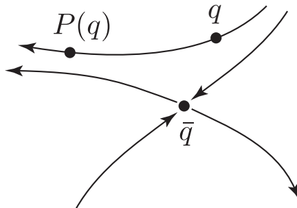
FIGURE 4.3.3. Poincaré map near a fixed point \bar{q} which is of saddle or hyperbolic type, i.e., nearby points evolve along hyperbolic curves.
