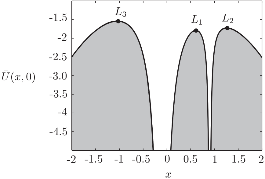
FIGURE 2.5.2. The graph of \bar{U}(x, 0) for \mu = 0.1 is shown. The solid line is the intersection of \bar{U}(x, y) in Figure 2.4.1 with the plane defined by y = 0 . At the x locations of m_1 and m_2 , the function plunges to -\infty . The maxima of \bar{U}(x, 0) correspond to the unstable collinear equilibrium points L_1, L_2 , and L_3 .
