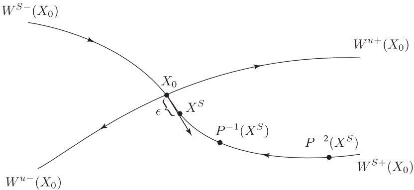
FIGURE 4.4.2. A simple way to compute an approximation of the two branches of the unstable ( W^{u\pm} ) or stable ( W^{s\pm} ) manifolds of a periodic orbit, which appear as manifolds to a fixed point in a Poincaré map P .
